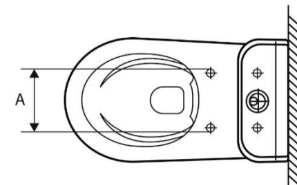
Stand-WC-Kombination
